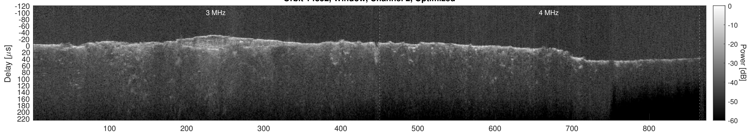
Orbit 14852, Cluttergram
