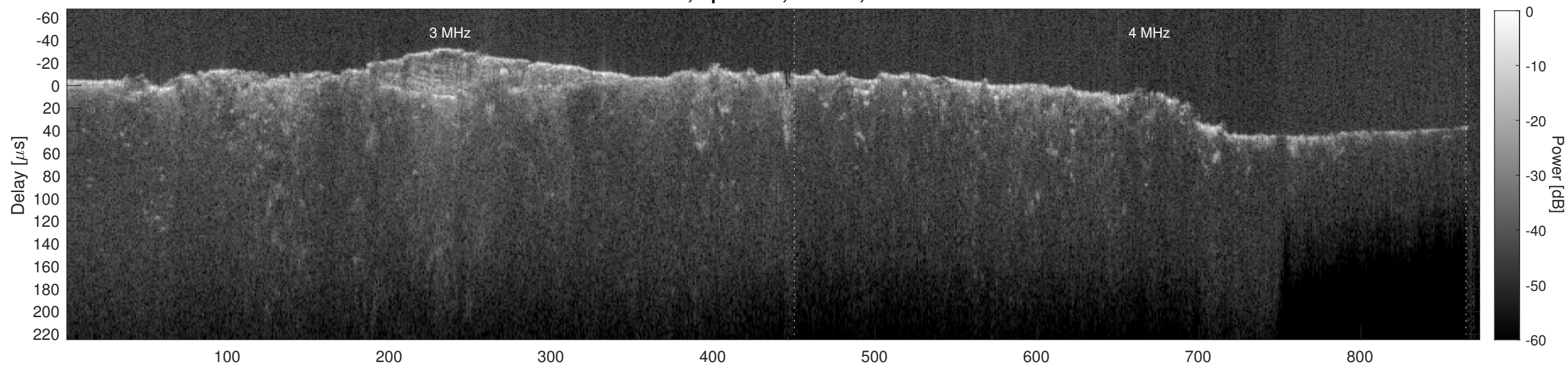
Orbit 14852, Cluttergram
