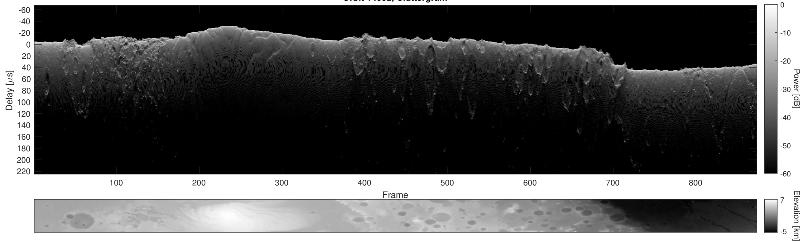
Orbit 14852, Cluttergram
