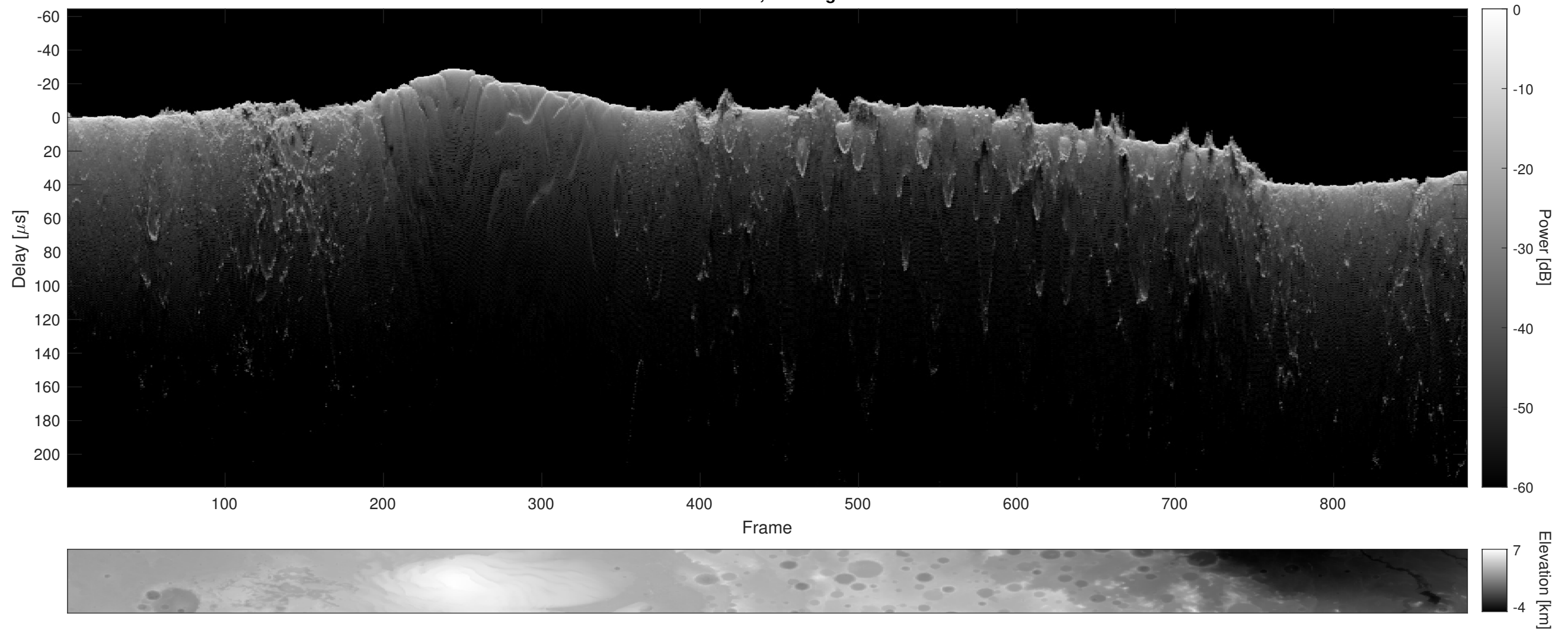
Orbit 14859, Cluttergram
