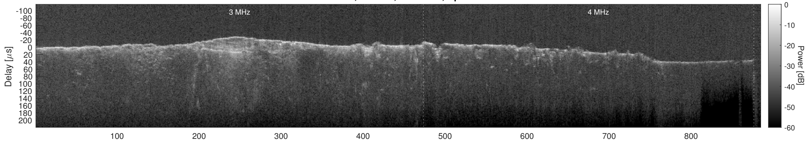
Orbit 14859, Cluttergram
