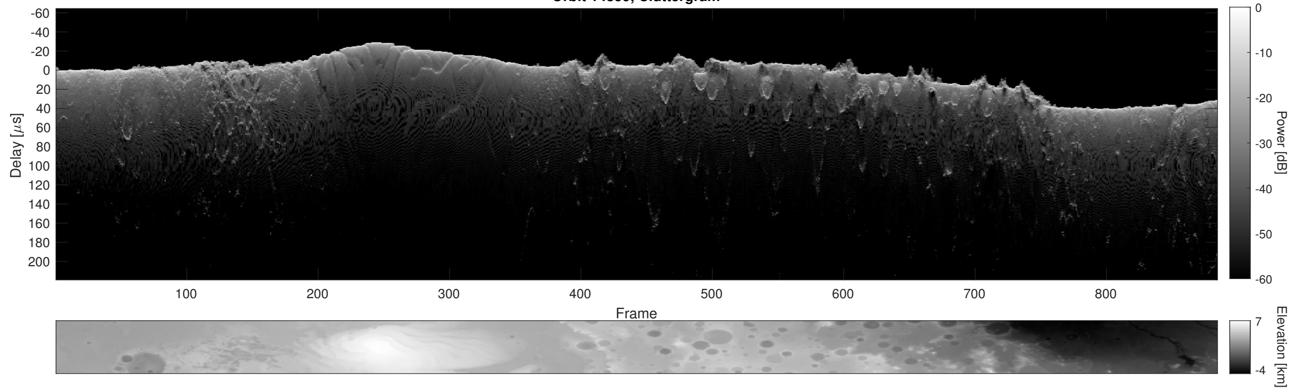
Orbit 14859, Cluttergram
