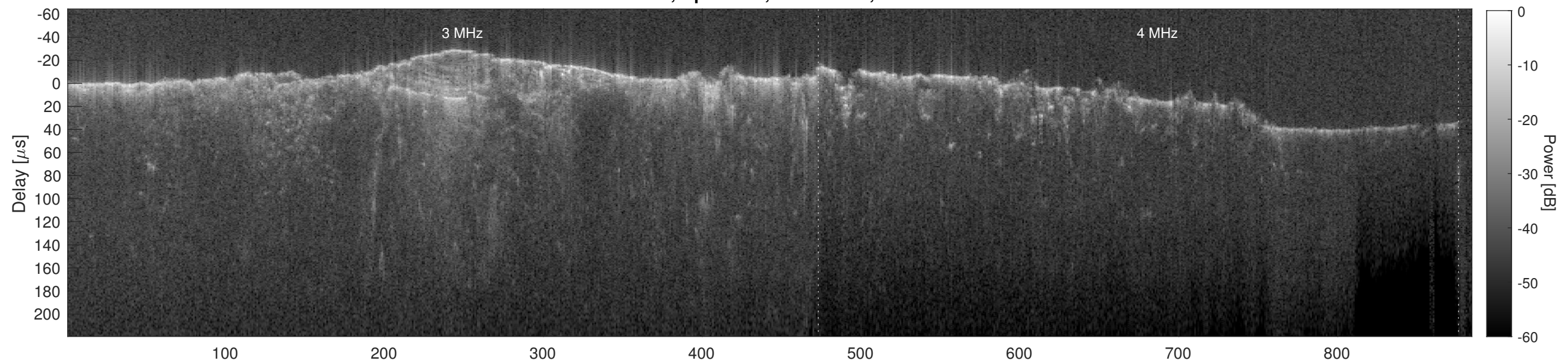
Orbit 14859, Cluttergram
