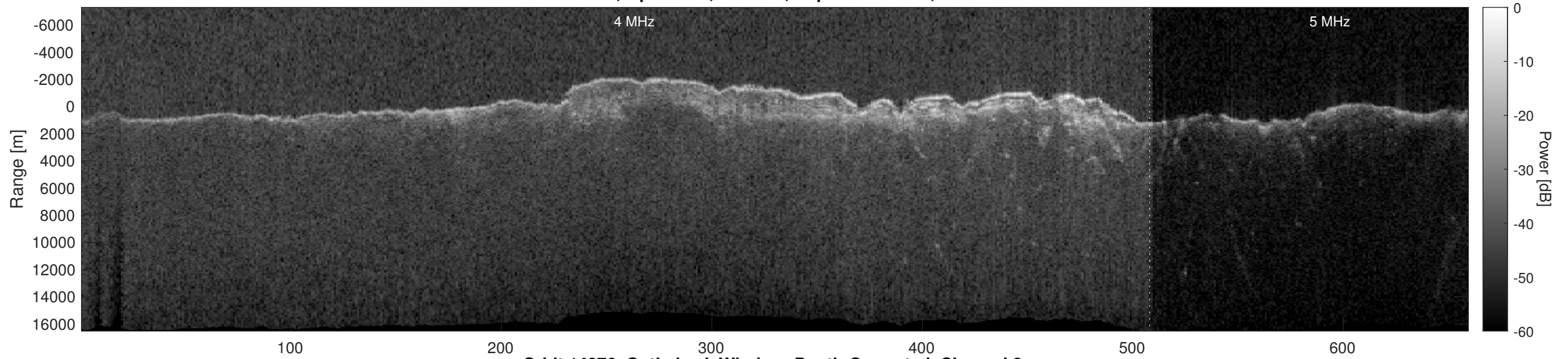
Orbit 14876, Optimized, Window, Depth-Corrected, Channel 2
