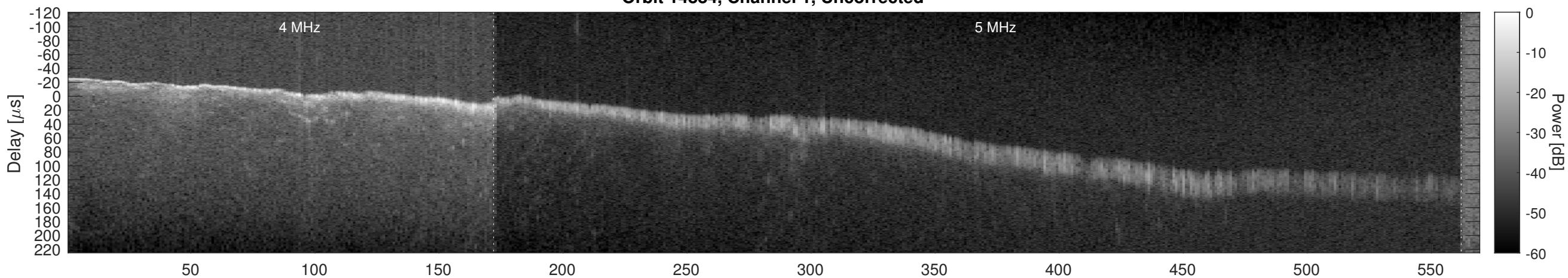
Orbit 14884, Window, Channel 1, Chapman
