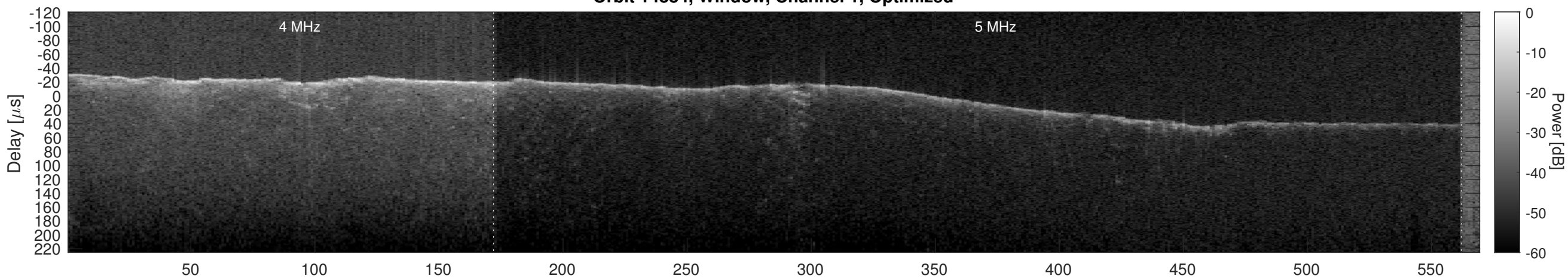
Orbit 14884, Cluttergram
