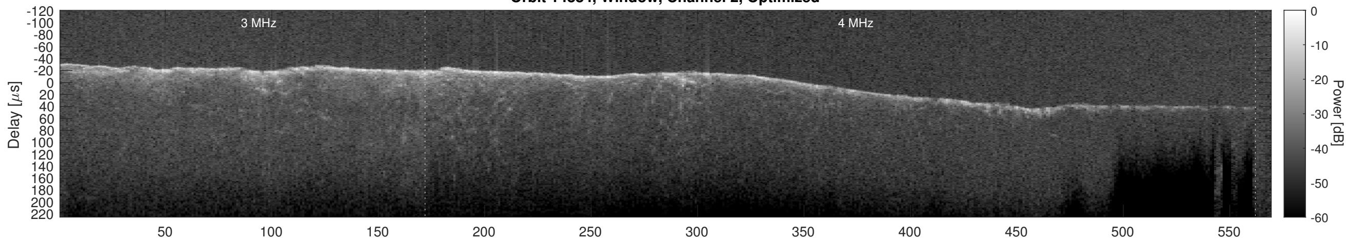
Orbit 14884, Cluttergram
