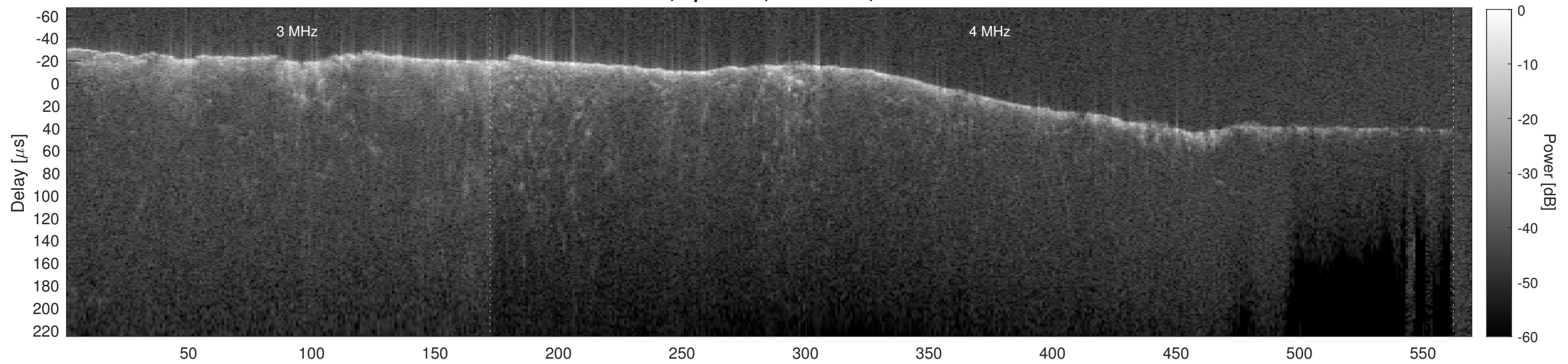
Orbit 14884, Cluttergram
