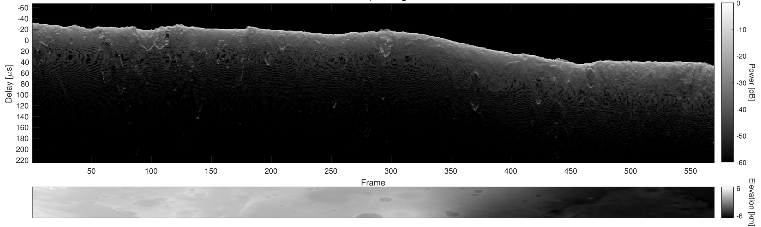
Orbit 14884, Cluttergram
