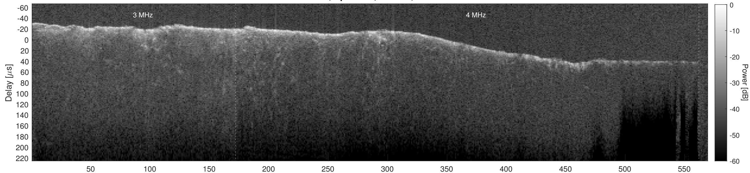
Orbit 14884, Cluttergram
