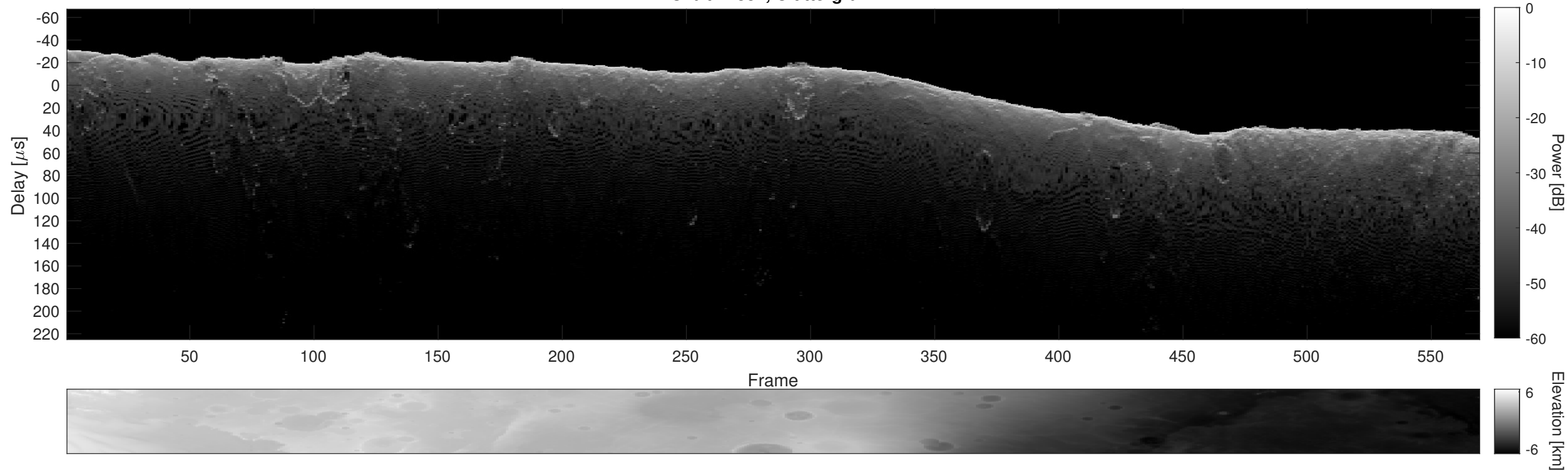
Orbit 14884, Cluttergram
