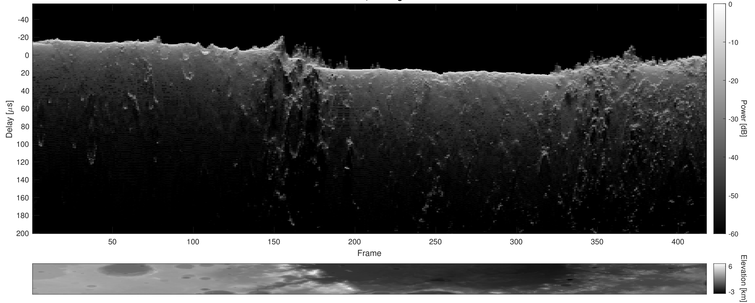
Orbit 14899, Cluttergram
