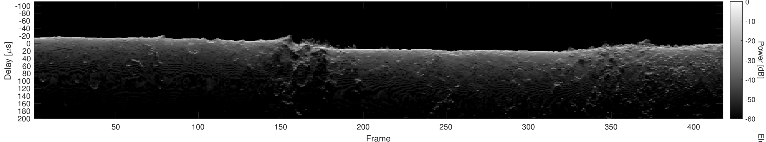
Orbit 14899, Cluttergram
