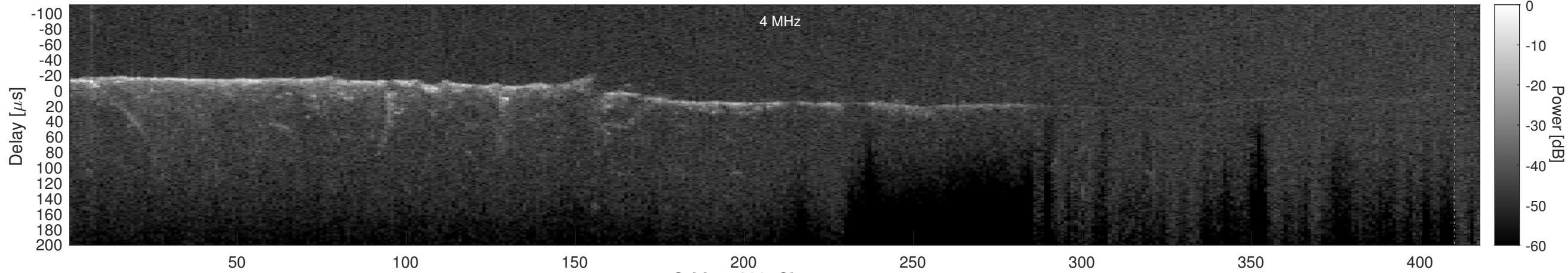
Orbit 14899, Cluttergram
