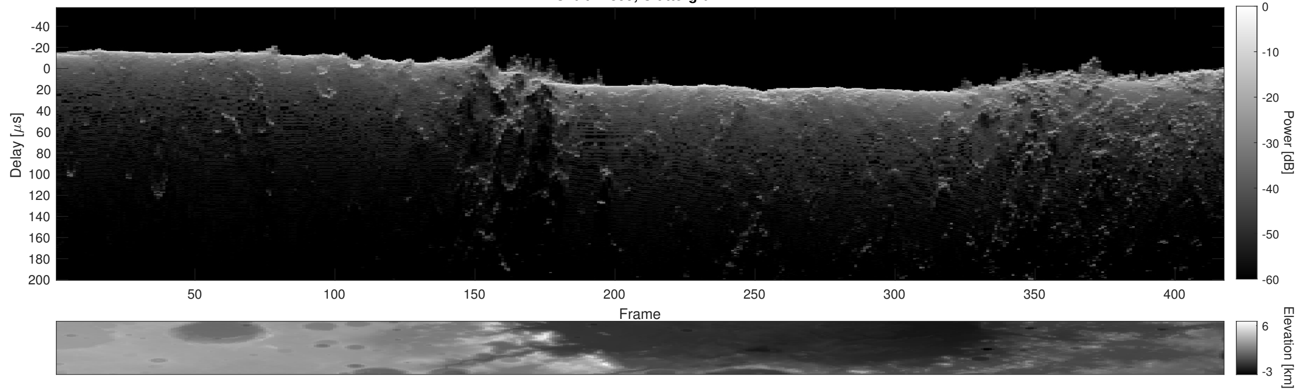
Orbit 14899, Cluttergram
