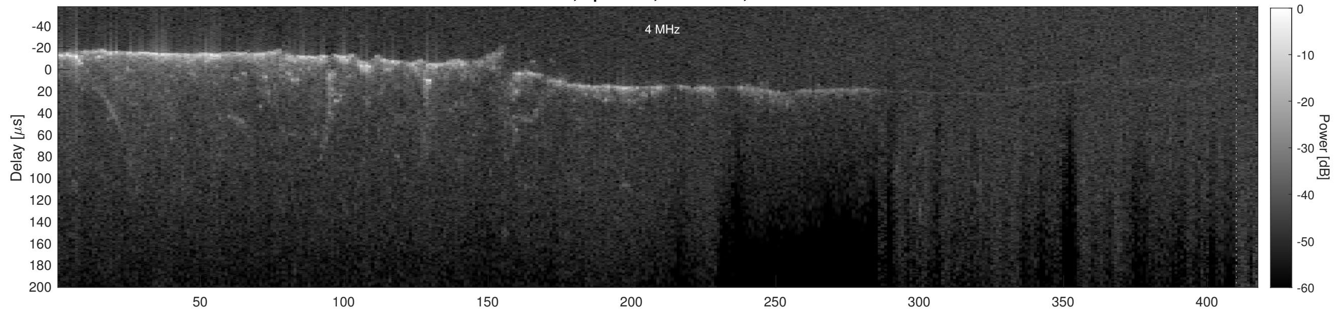
Orbit 14899, Cluttergram
