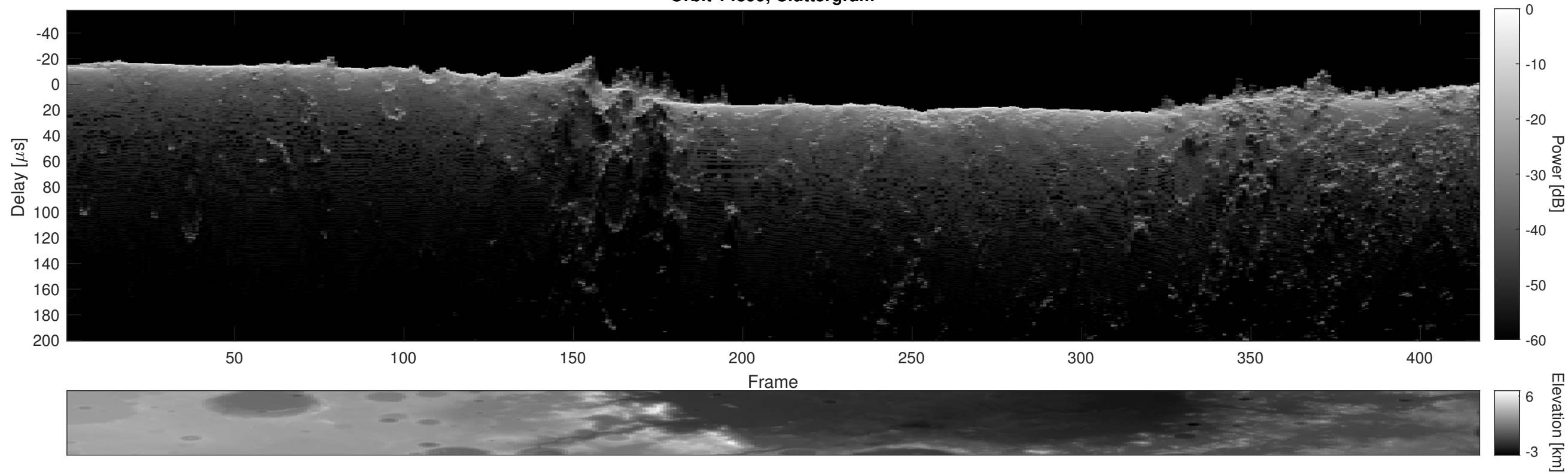
Orbit 14899, Cluttergram
