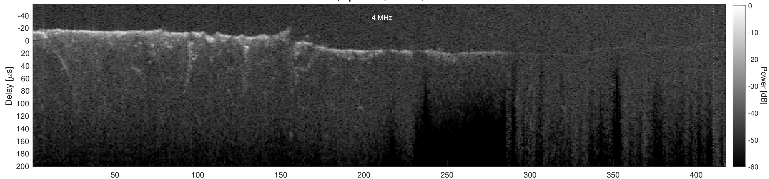
Orbit 14899, Cluttergram
