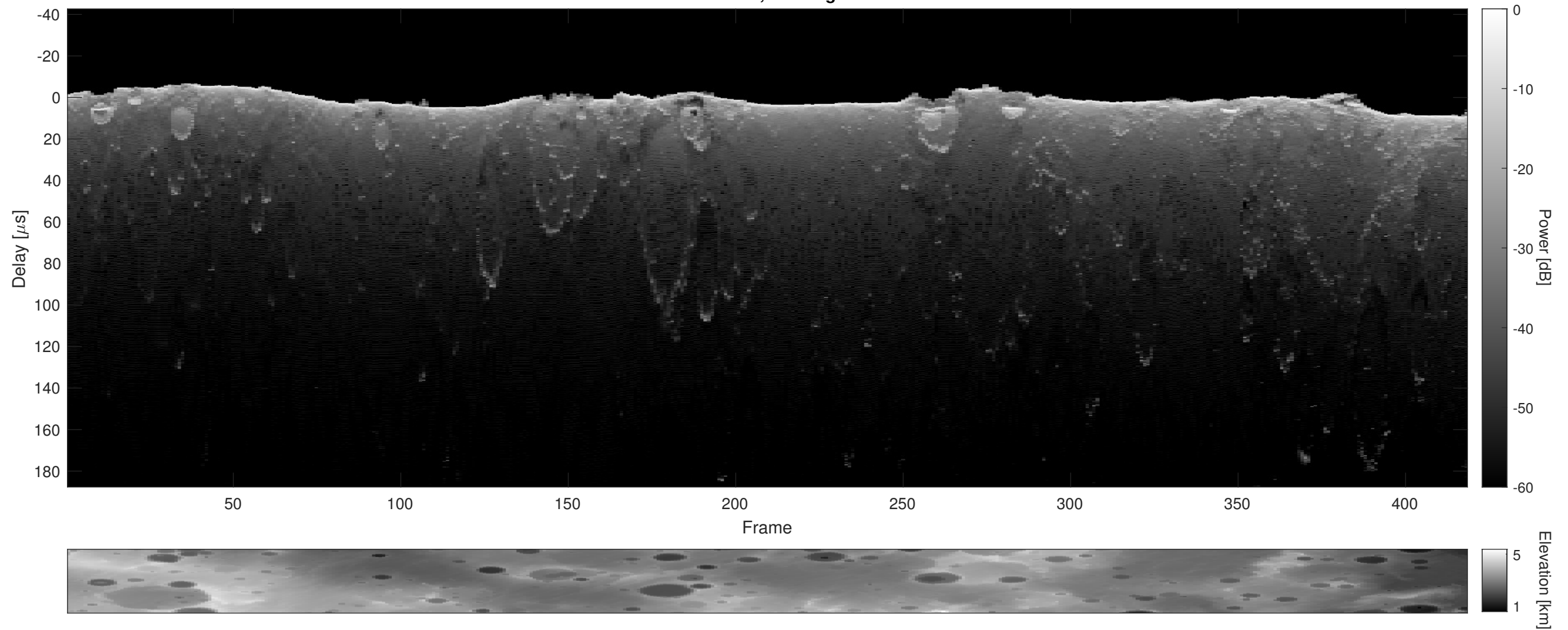
Orbit 14900, Cluttergram
