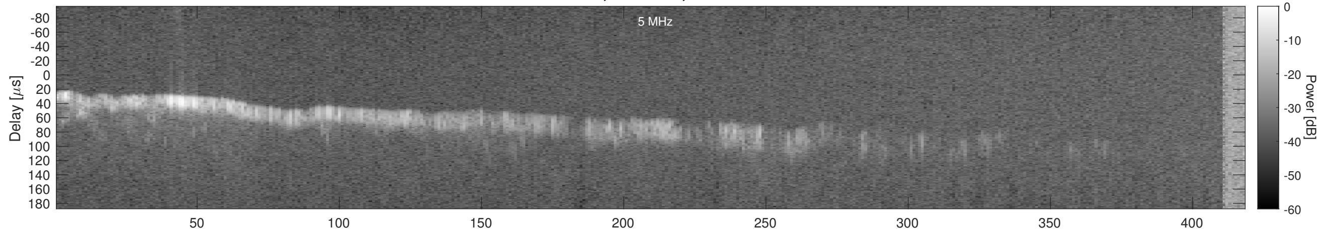
Orbit 14900, Window, Channel 1, Chapman
