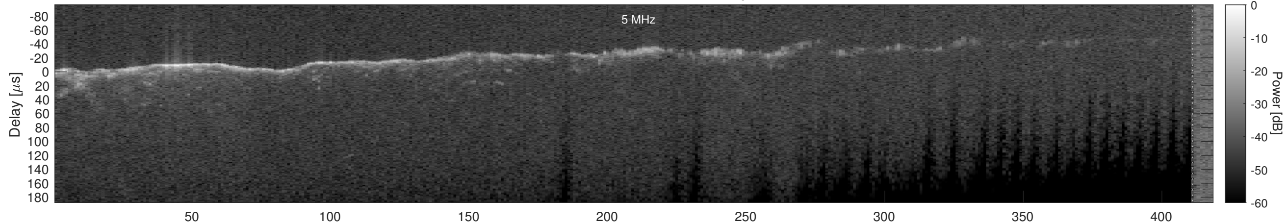
Orbit 14900, Window, Channel 1, Optimized
