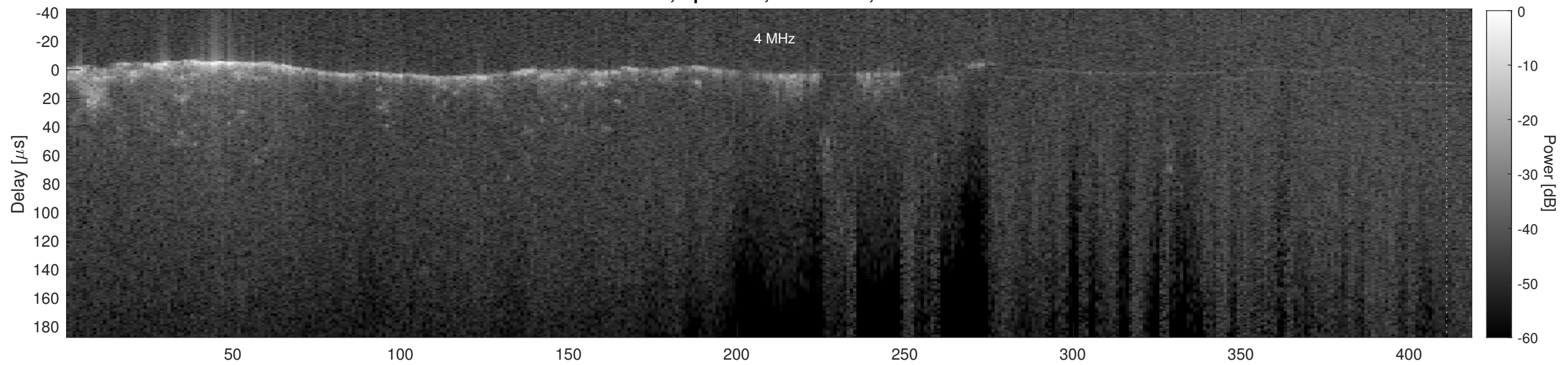
Orbit 14900, Cluttergram
