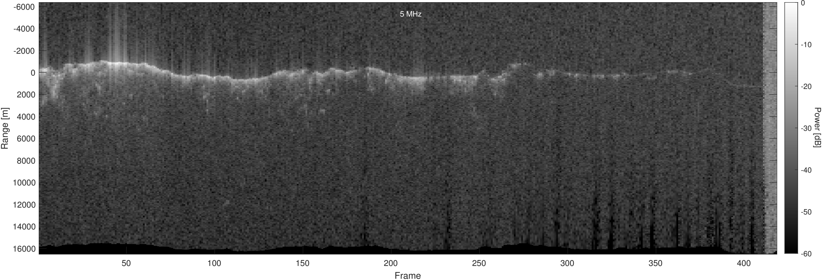
Orbit 14900, Optimized, No Window, Depth-Corrected, Channel 2
