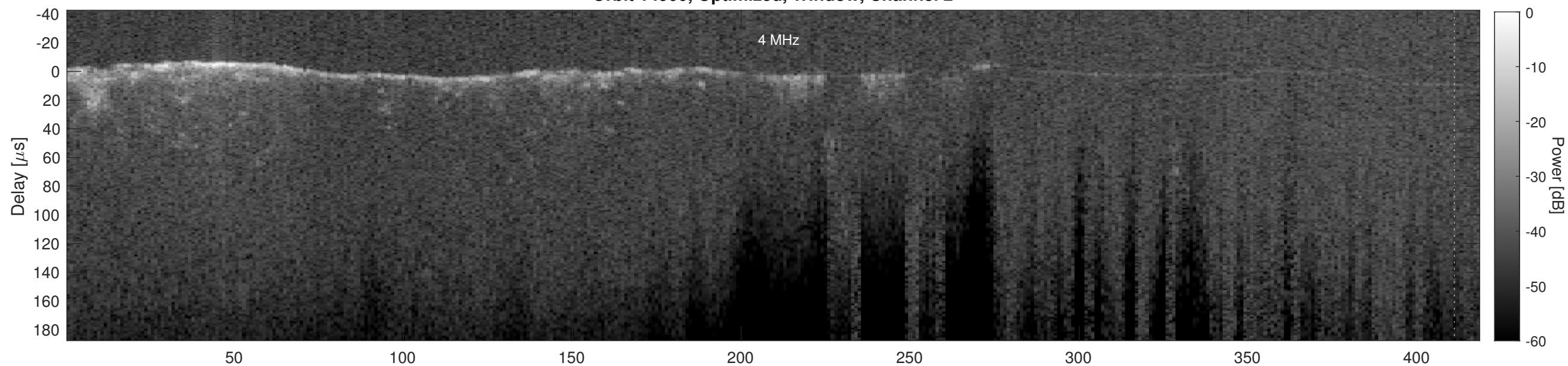
Orbit 14900, Cluttergram
