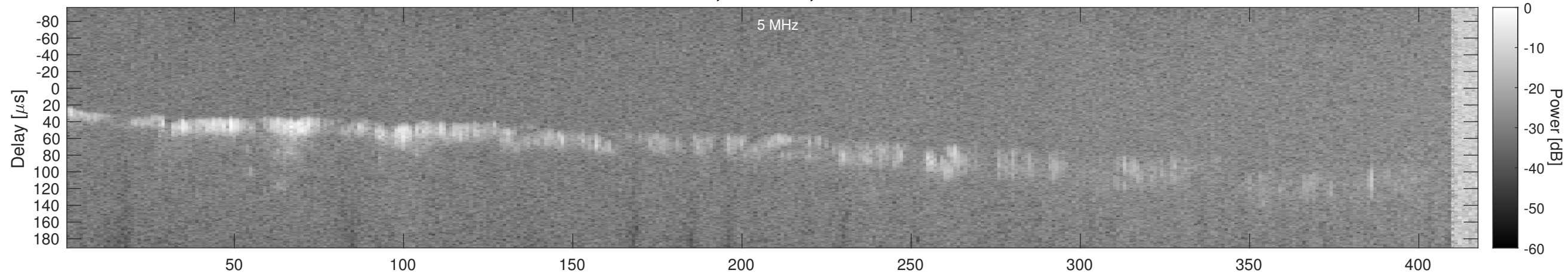
Orbit 14904, Window, Channel 1, Chapman
