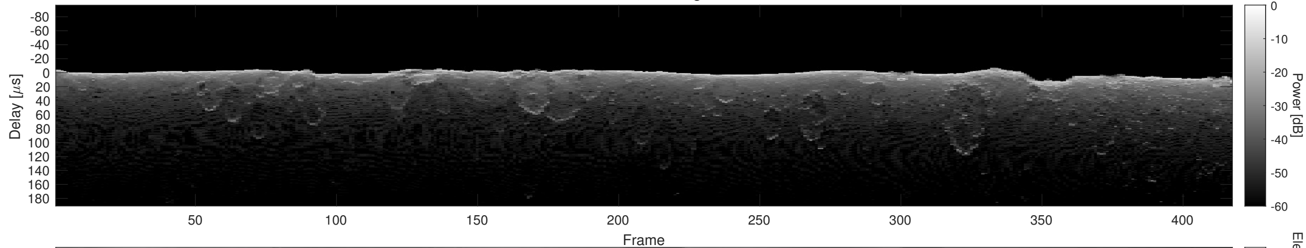
Orbit 14904, Cluttergram
