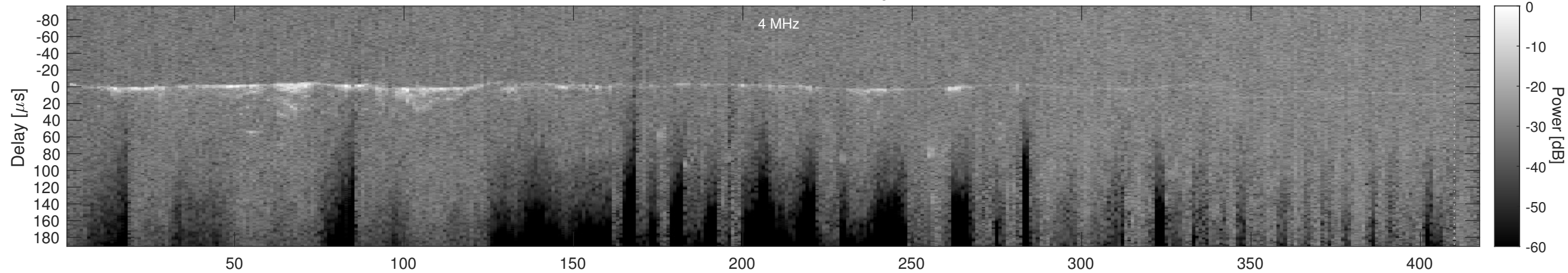
Orbit 14904, Cluttergram
