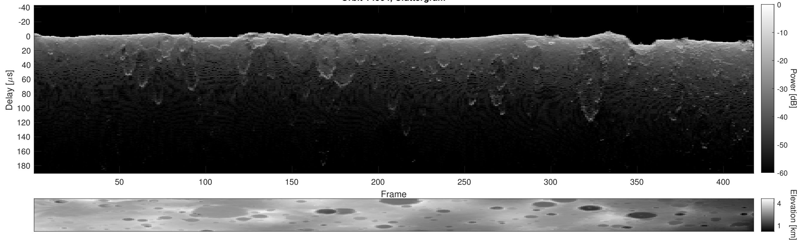
Orbit 14904, Cluttergram
