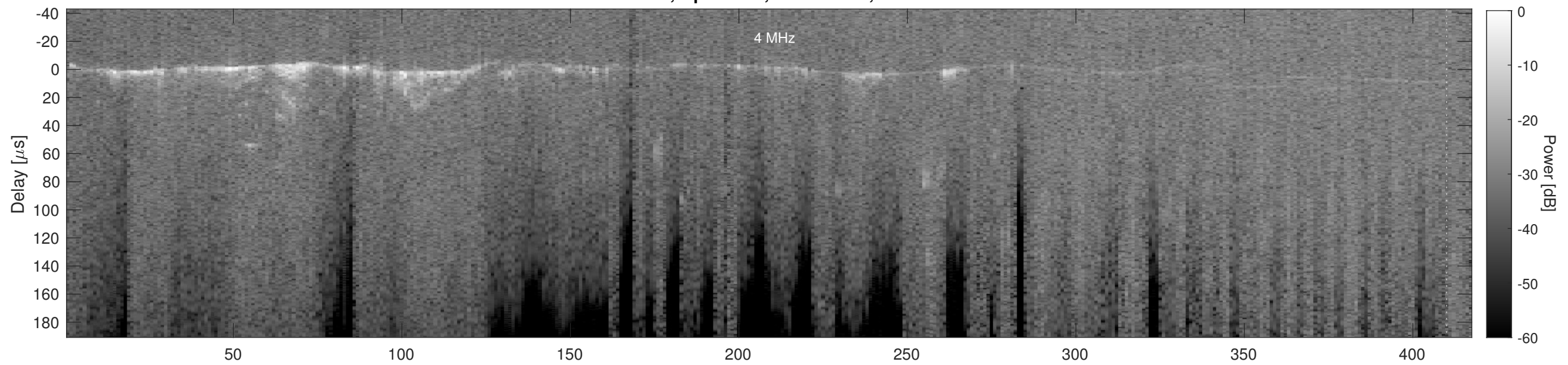
Orbit 14904, Cluttergram
