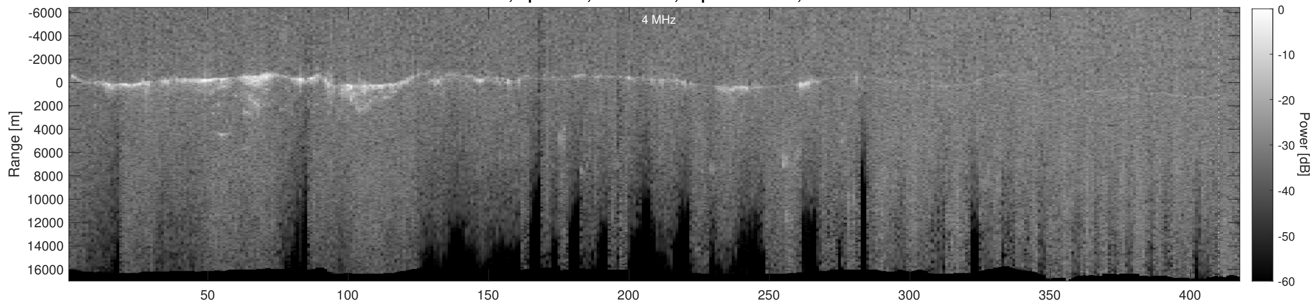
Orbit 14904, Depth-Corrected Cluttergram
