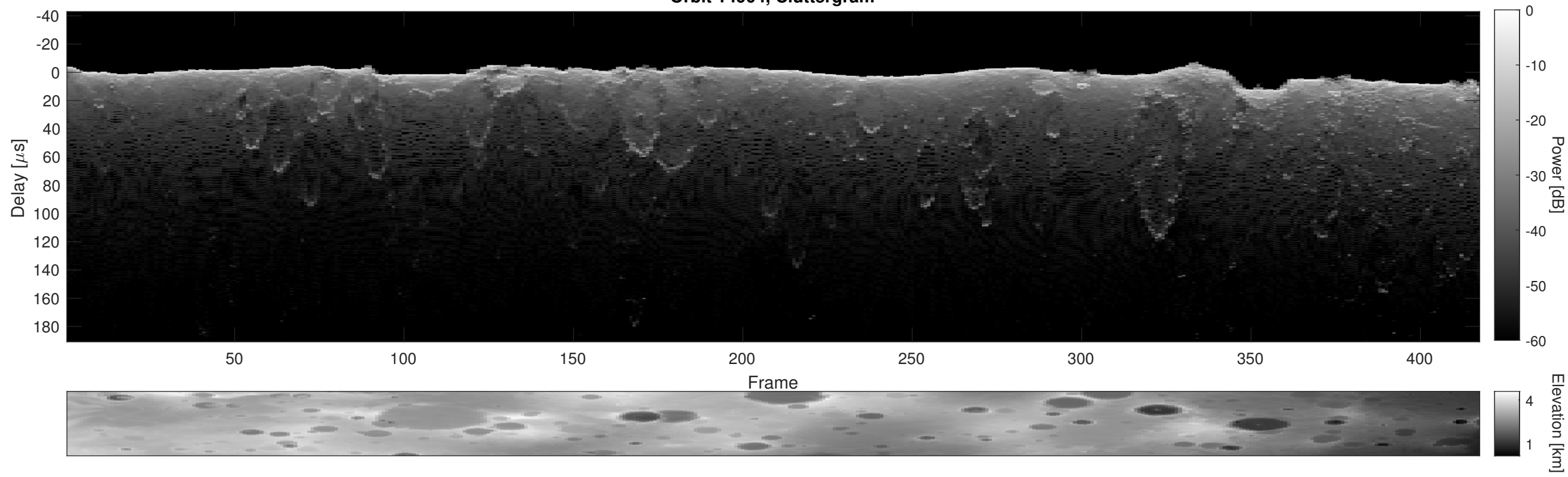
Orbit 14904, Cluttergram
