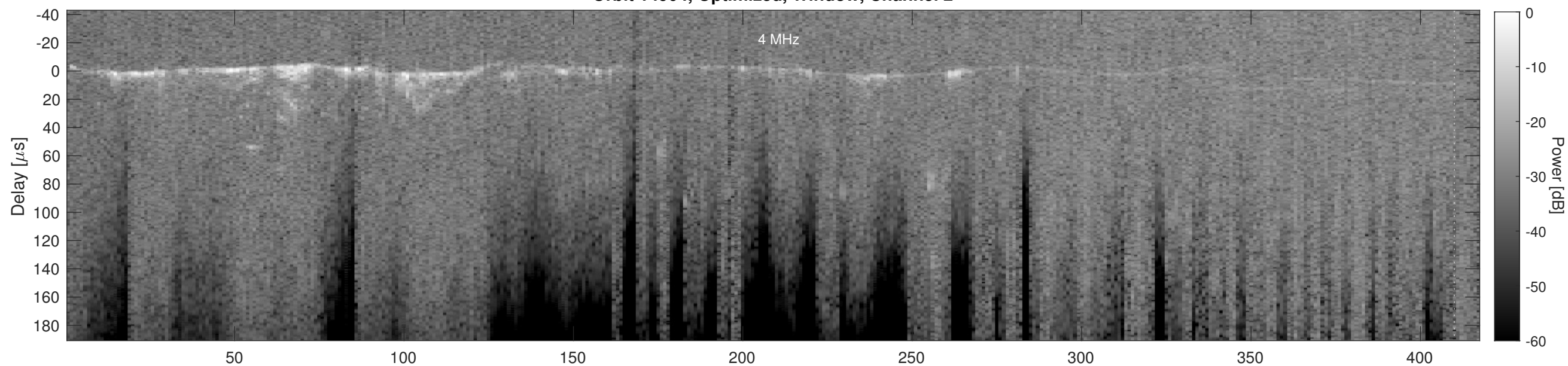
Orbit 14904, Cluttergram
