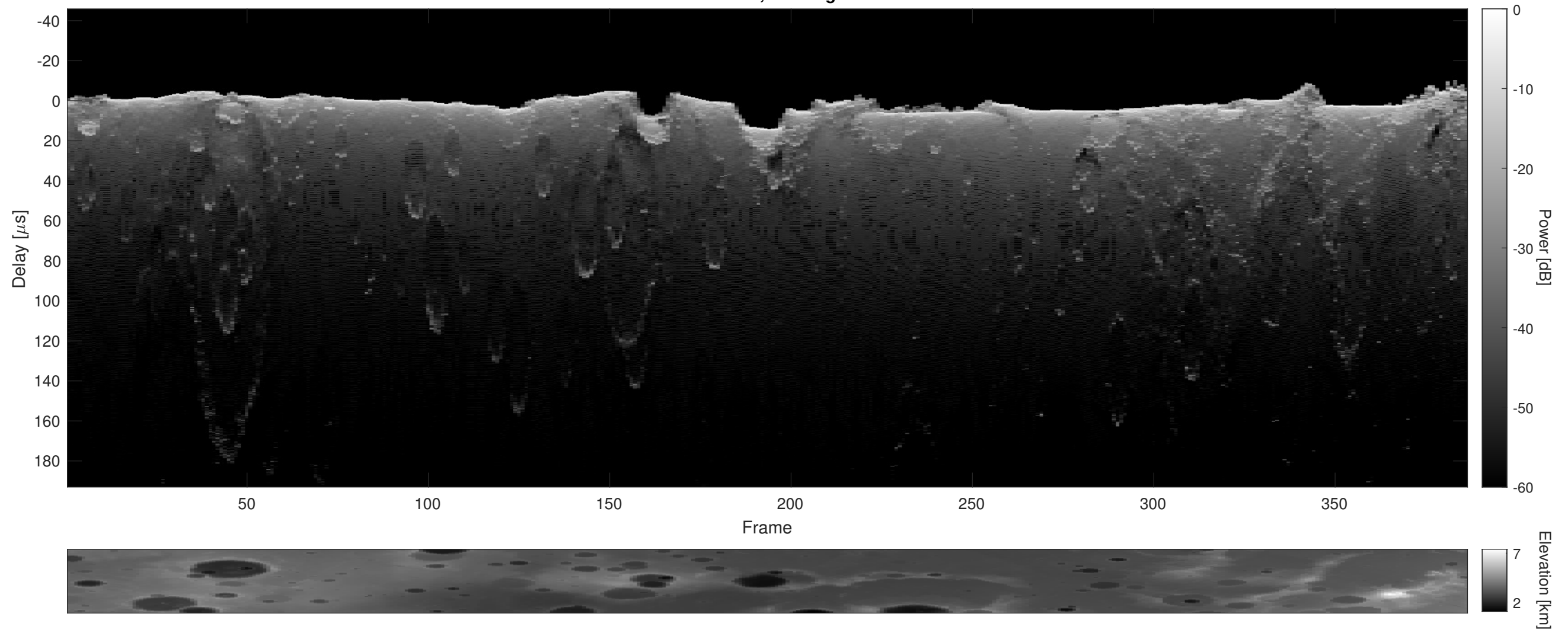
Orbit 14935, Cluttergram
