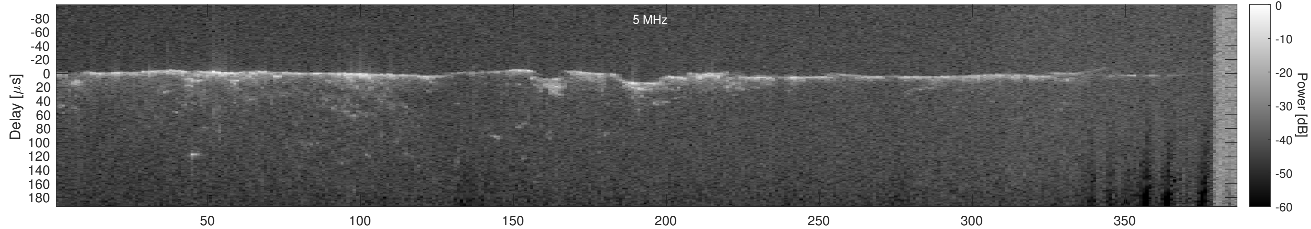
Orbit 14935, Cluttergram
