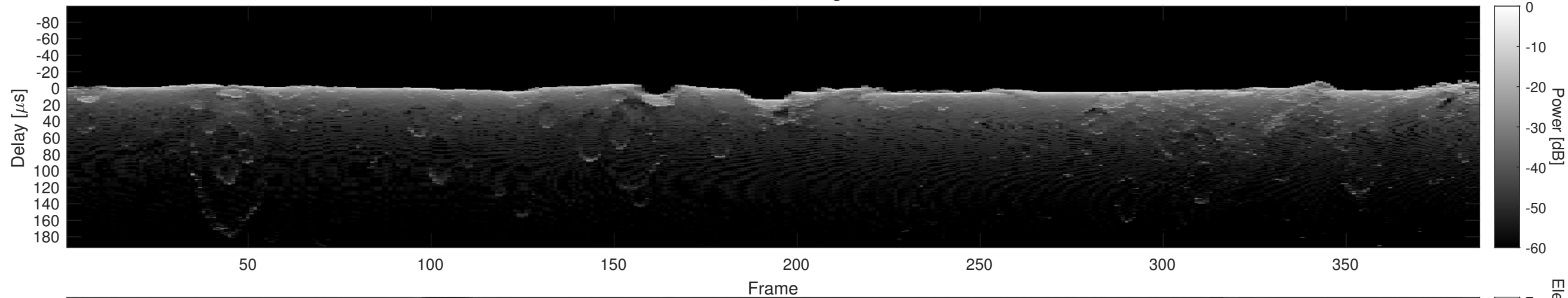
Orbit 14935, Cluttergram
