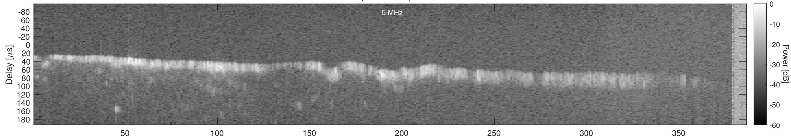
Orbit 14935, Window, Channel 1, Chapman
