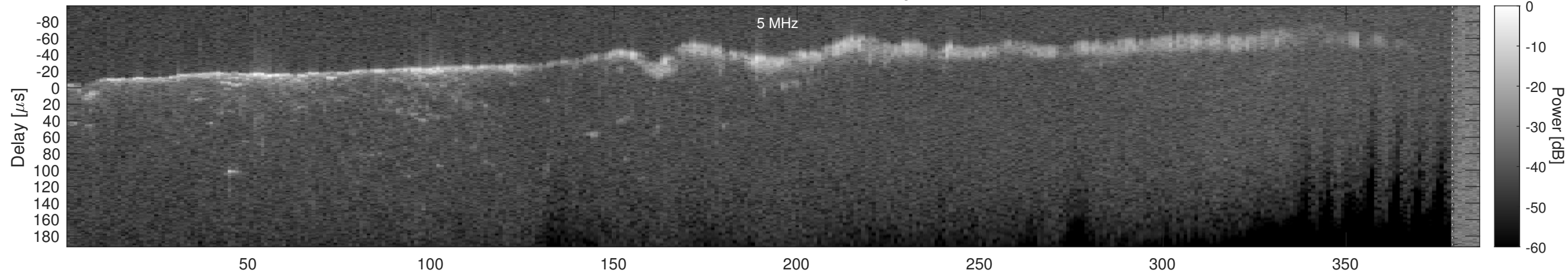
Orbit 14935, Window, Channel 1, Optimized
