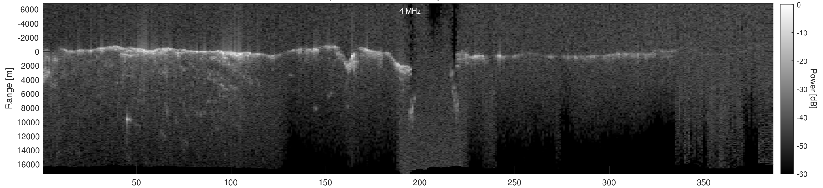
Orbit 14935, Depth-Corrected Cluttergram
