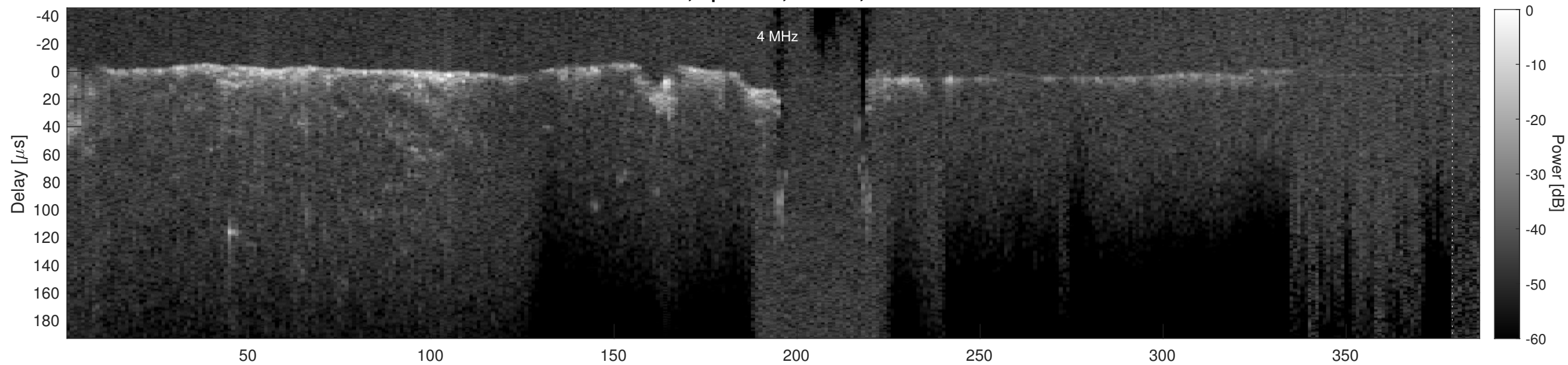
Orbit 14935, Cluttergram
