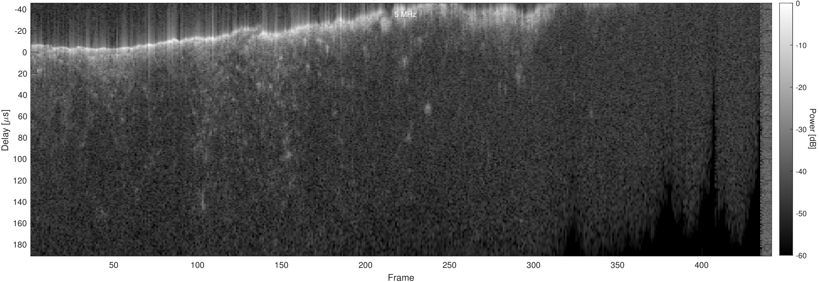
Orbit 14938, Chapman, No Window, Channel 2
