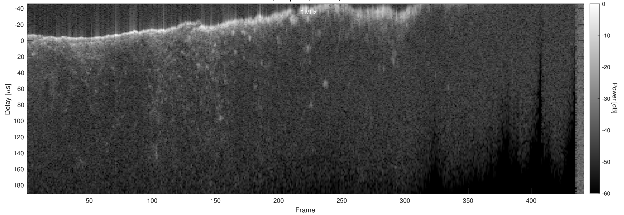
Orbit 14938, Chapman, Window, Channel 2
