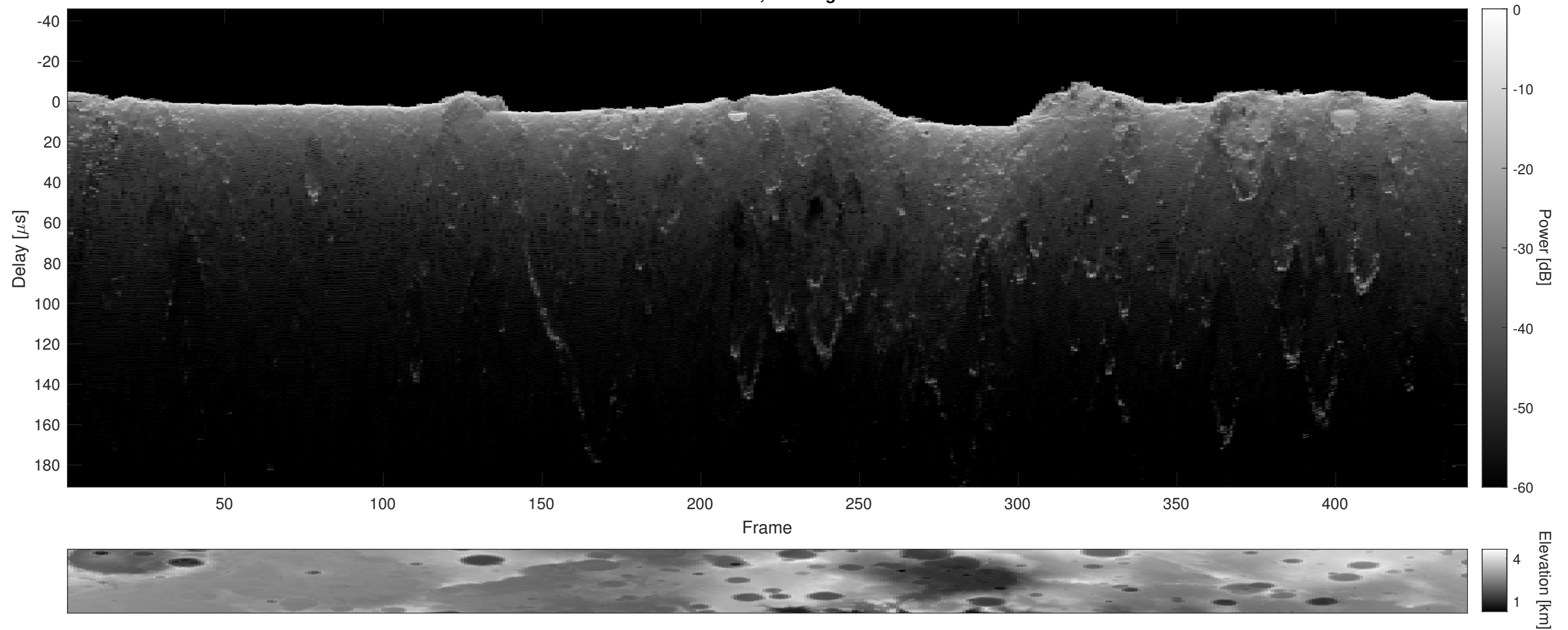
Orbit 14938, Cluttergram
