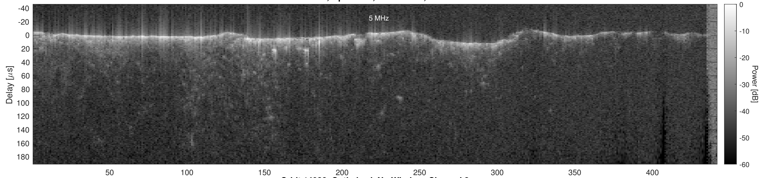
Orbit 14938, Optimized, No Window, Channel 2
