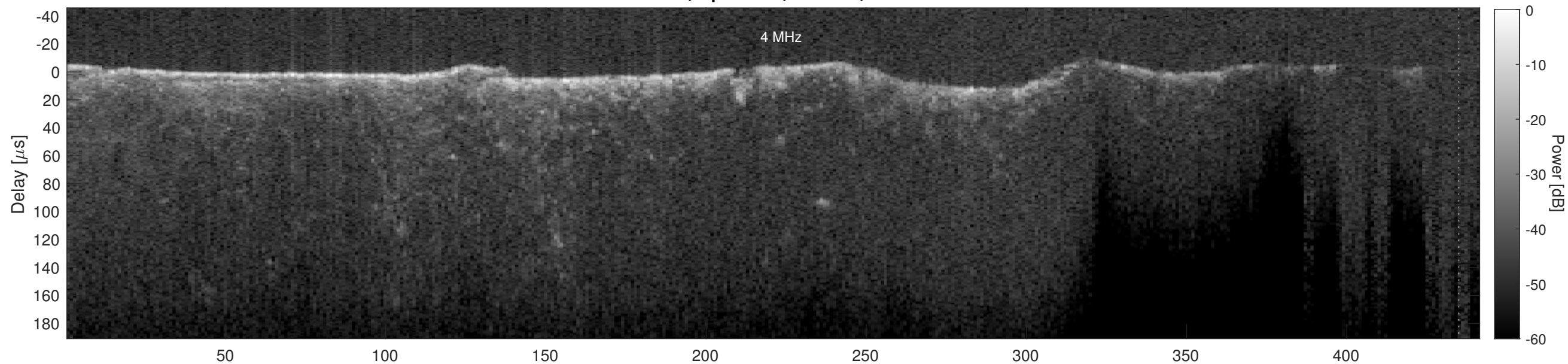
Orbit 14938, Cluttergram
