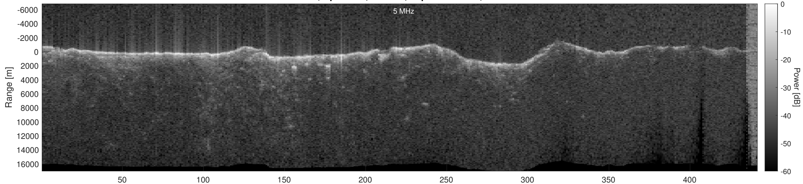
Orbit 14938, Optimized, Window, Depth-Corrected, Channel 2
