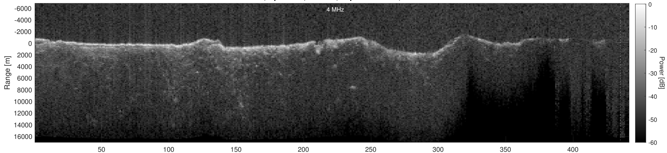
Orbit 14938, Depth-Corrected Cluttergram
