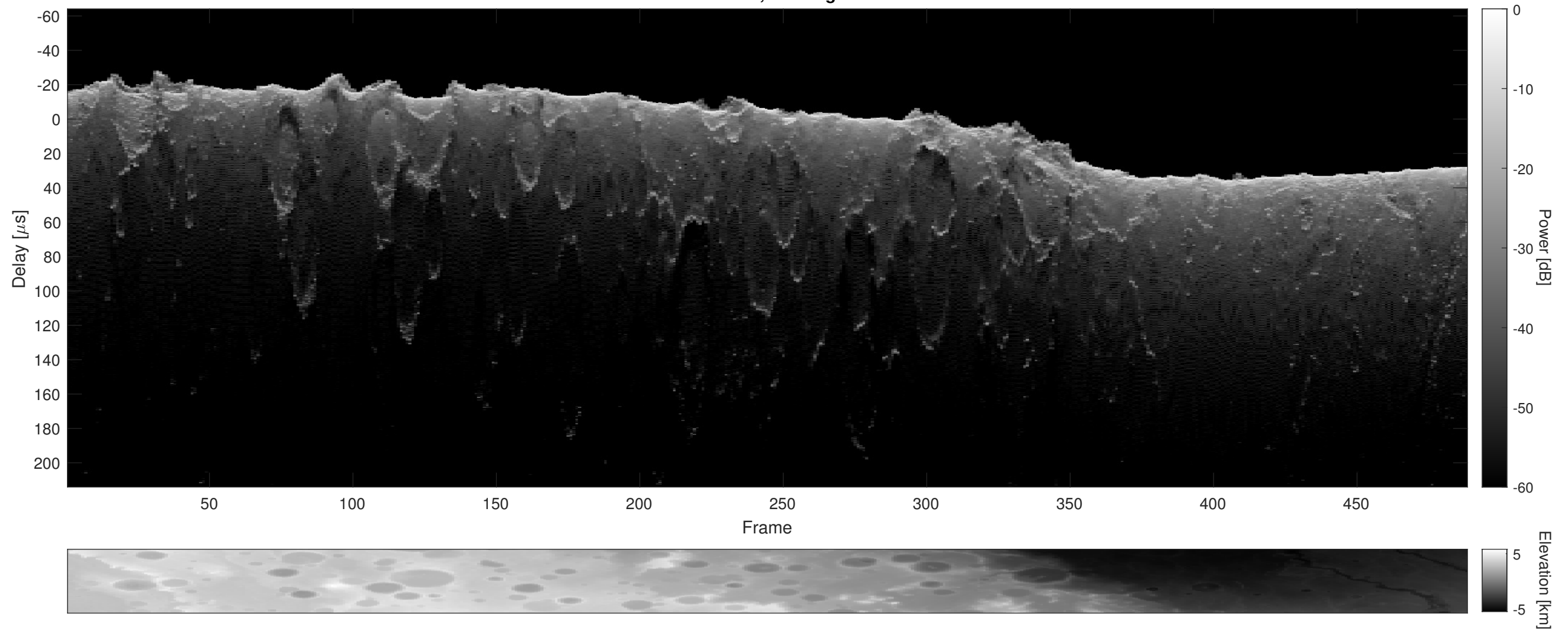
Orbit 14940, Cluttergram
