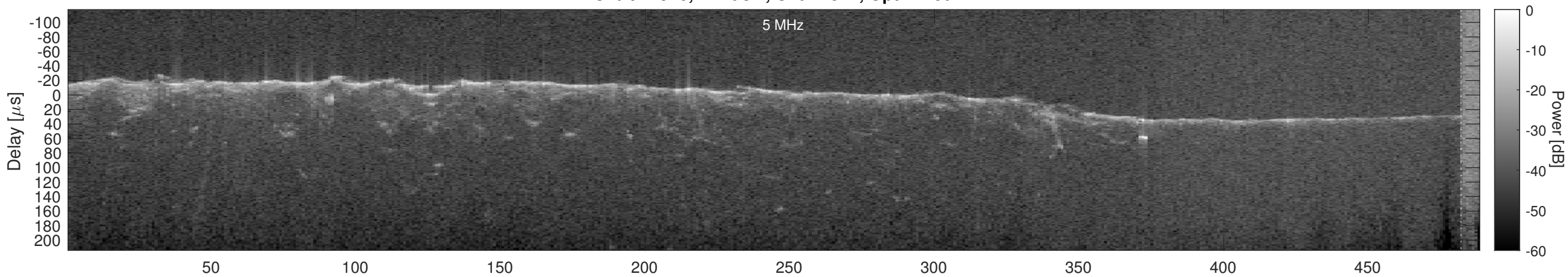
Orbit 14940, Cluttergram
