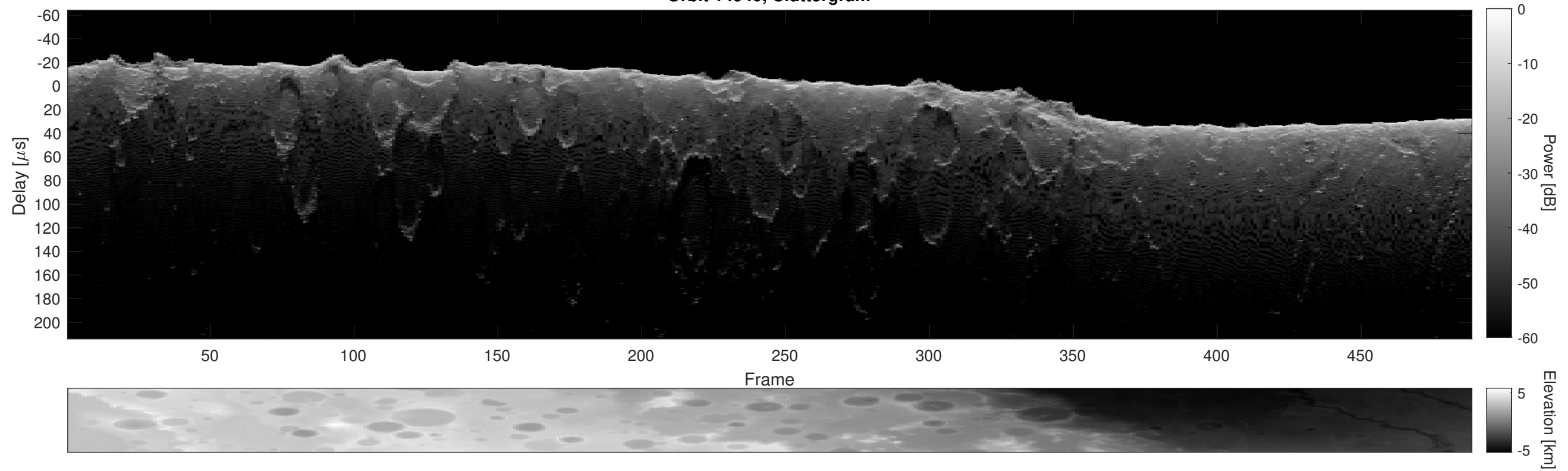
Orbit 14940, Cluttergram
