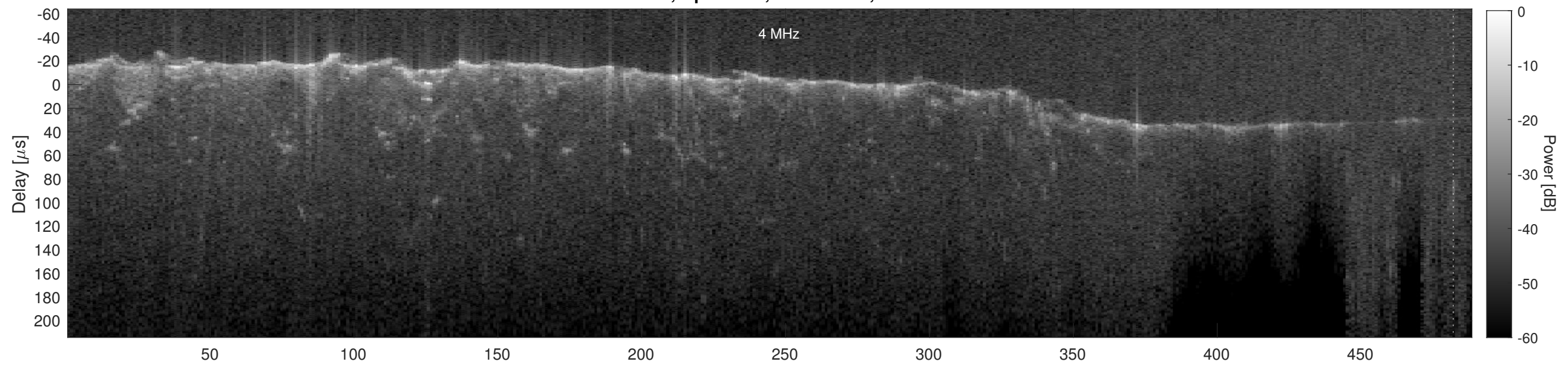
Orbit 14940, Cluttergram
