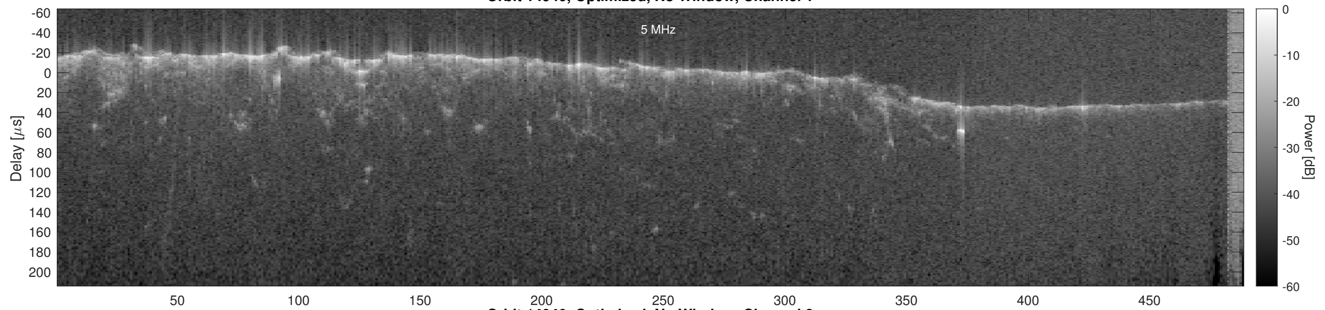
Orbit 14940, Optimized, No Window, Channel 2
