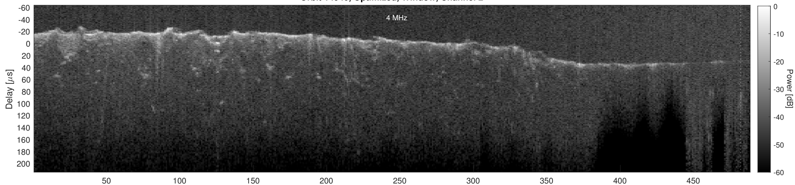
Orbit 14940, Cluttergram
