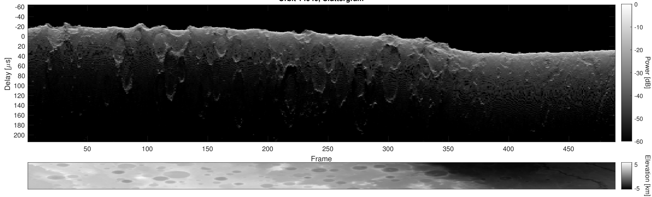
Orbit 14940, Cluttergram
