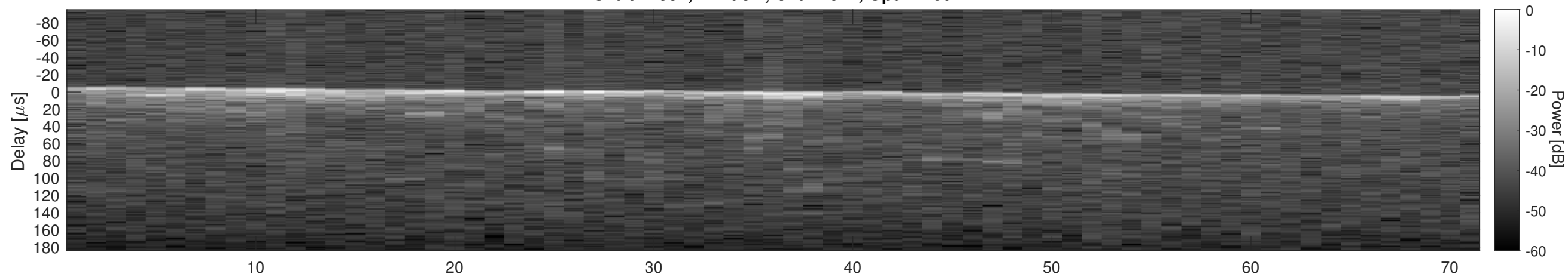
Orbit 14951, Cluttergram
