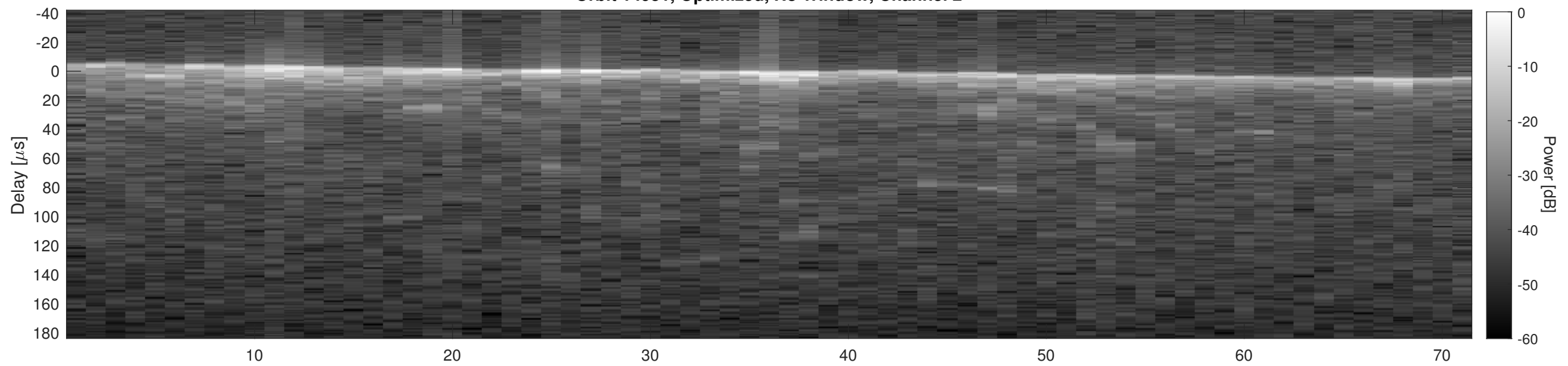
Orbit 14951, Cluttergram
