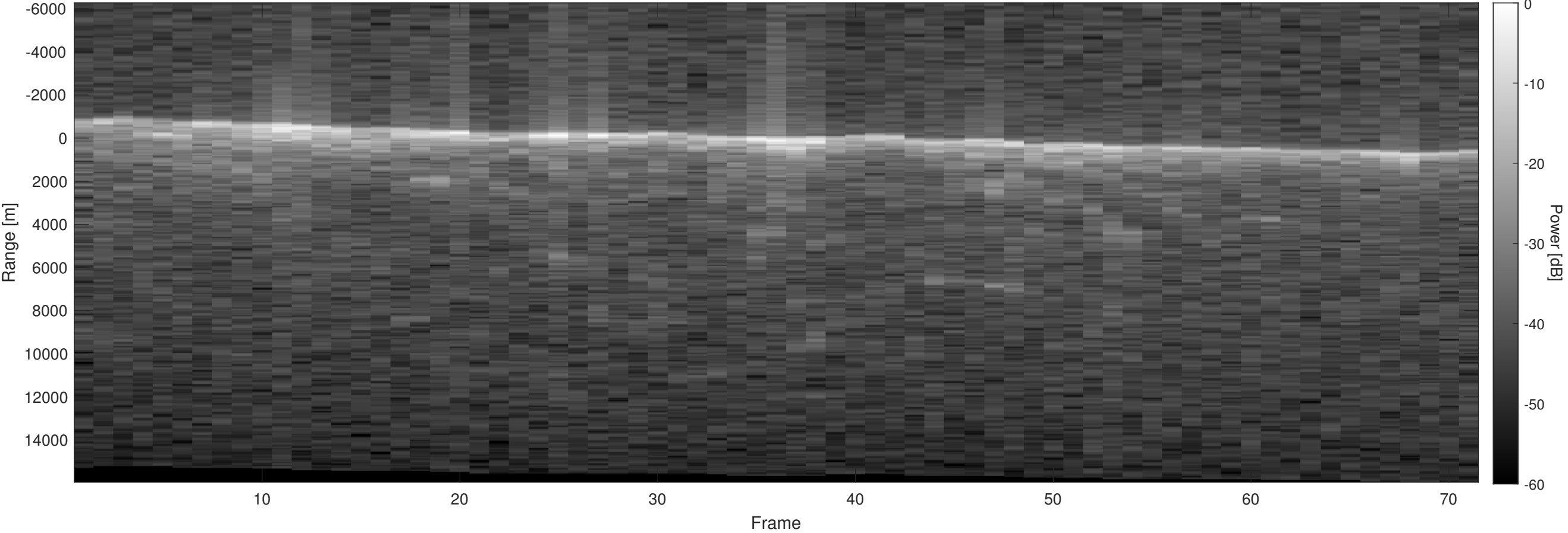
Orbit 14951, Optimized, No Window, Depth-Corrected, Channel 2
