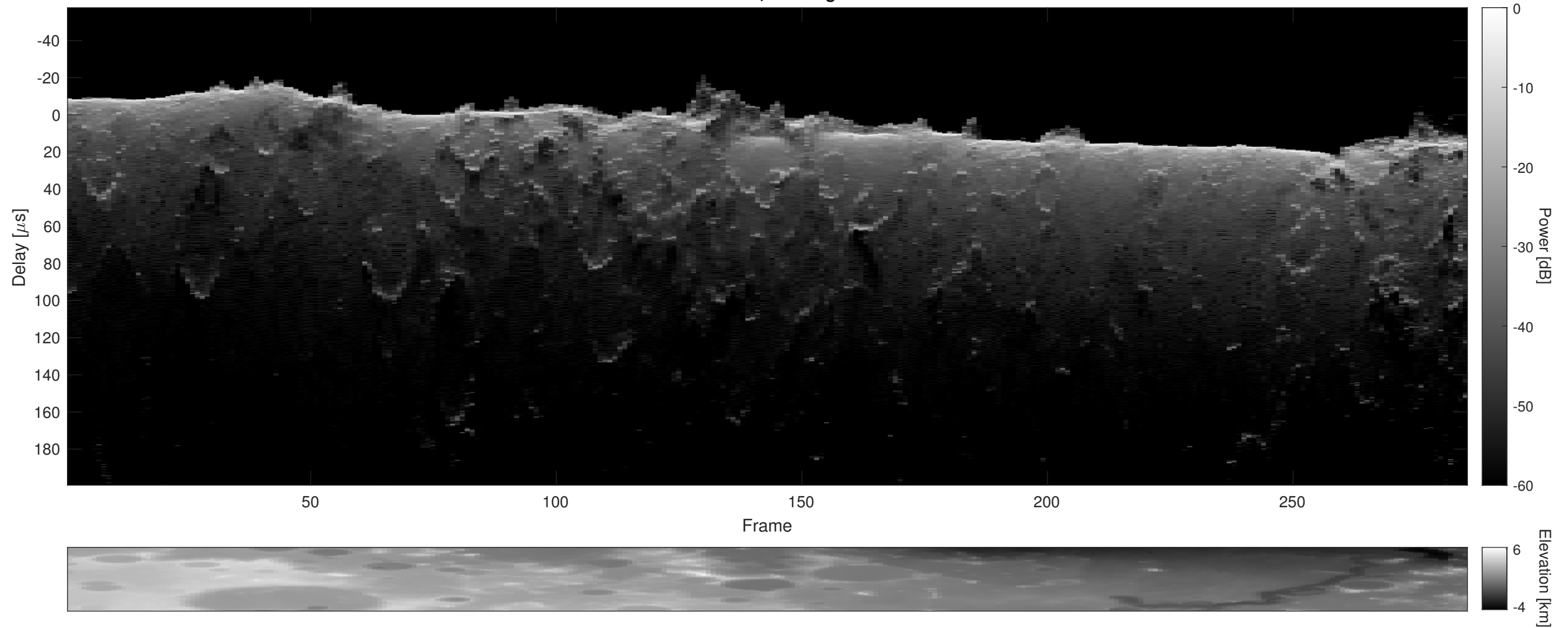
Orbit 14954, Cluttergram
