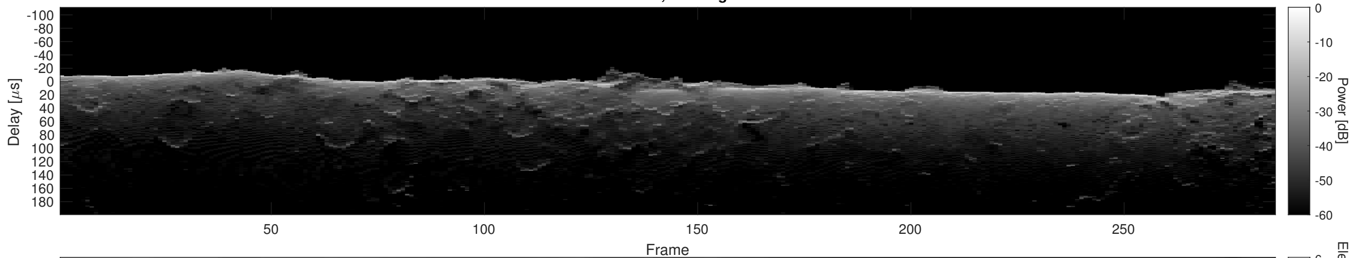
Orbit 14954, Cluttergram
