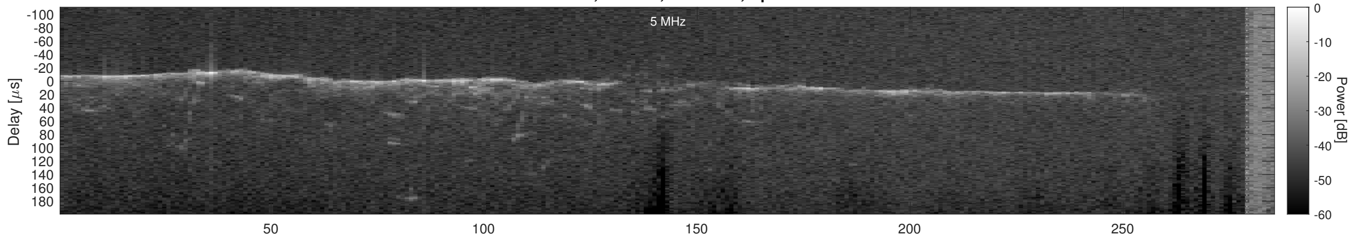
Orbit 14954, Cluttergram
