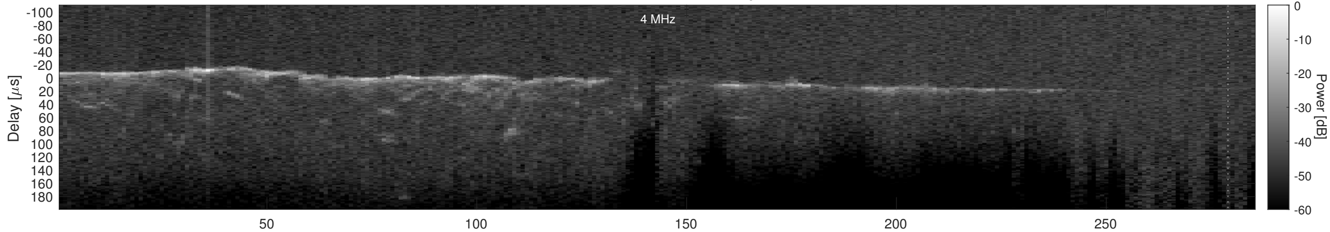
Orbit 14954, Cluttergram
