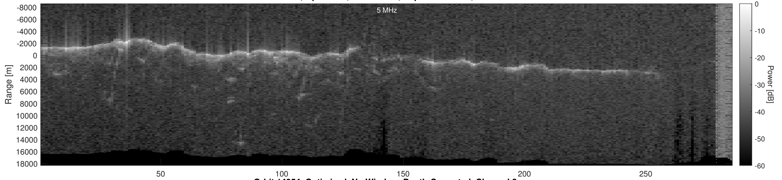
Orbit 14954, Optimized, No Window, Depth-Corrected, Channel 2
