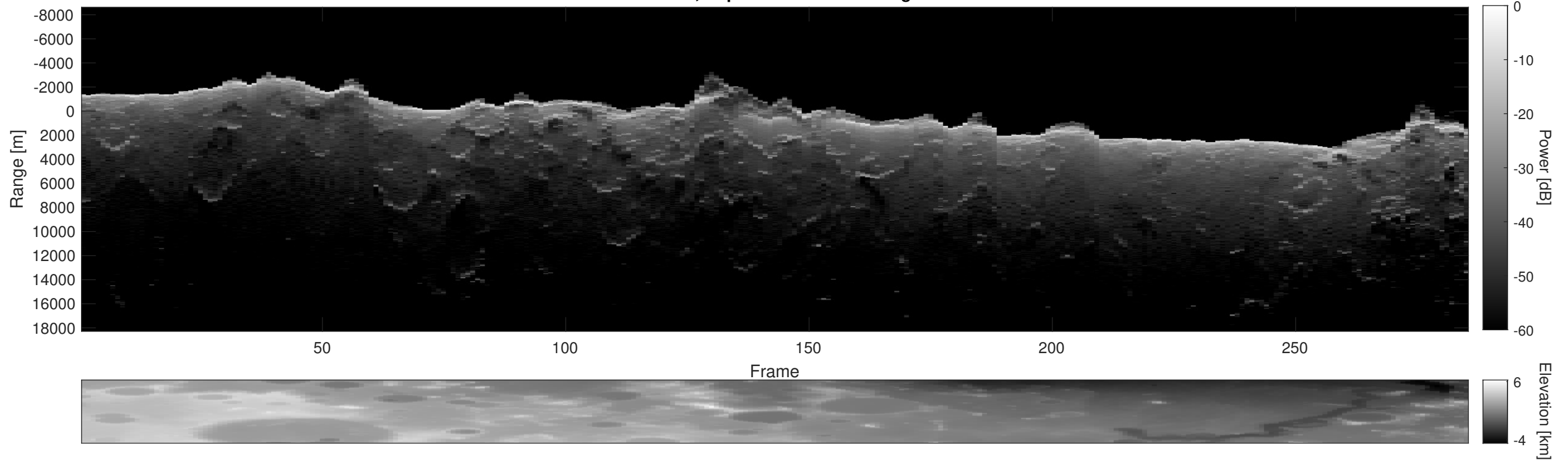
Orbit 14954, Depth-Corrected Cluttergram
