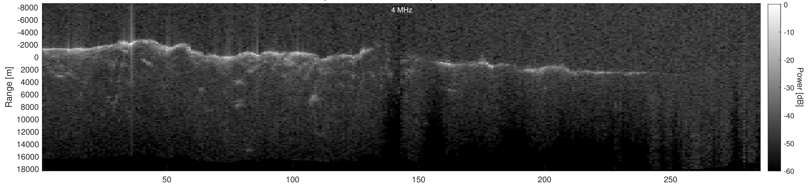
Orbit 14954, Depth-Corrected Cluttergram
