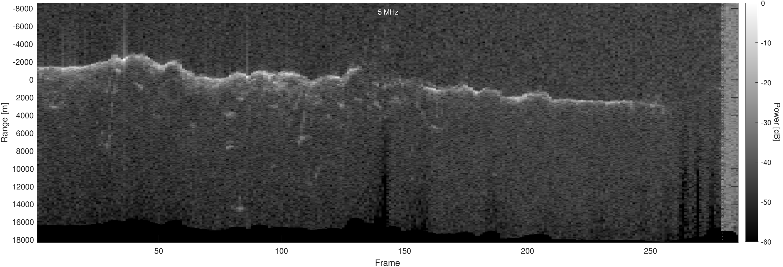
Orbit 14954, Optimized, Window, Depth-Corrected, Channel 2
