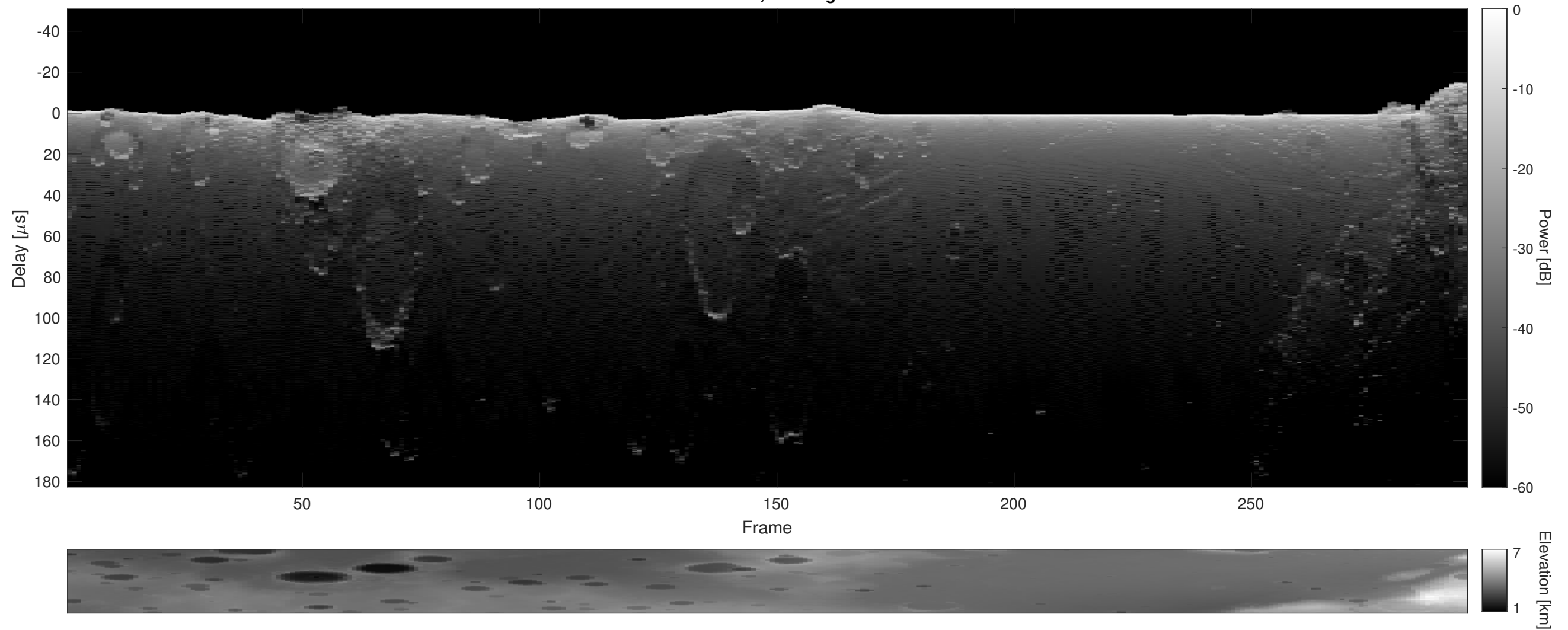
Orbit 14956, Cluttergram
