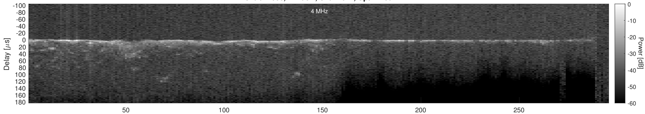
Orbit 14956, Cluttergram
