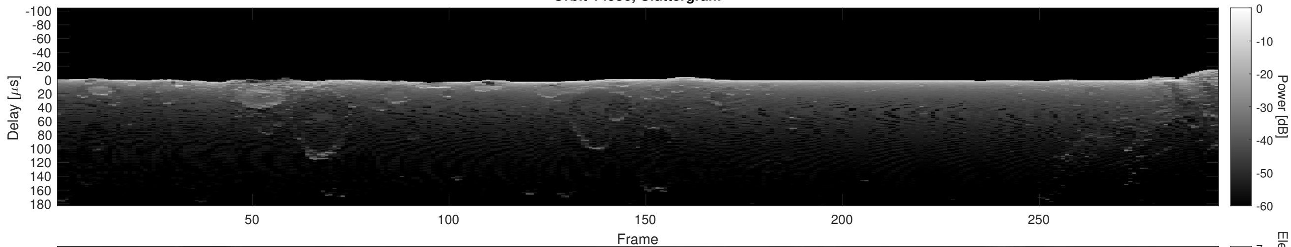
Orbit 14956, Cluttergram
