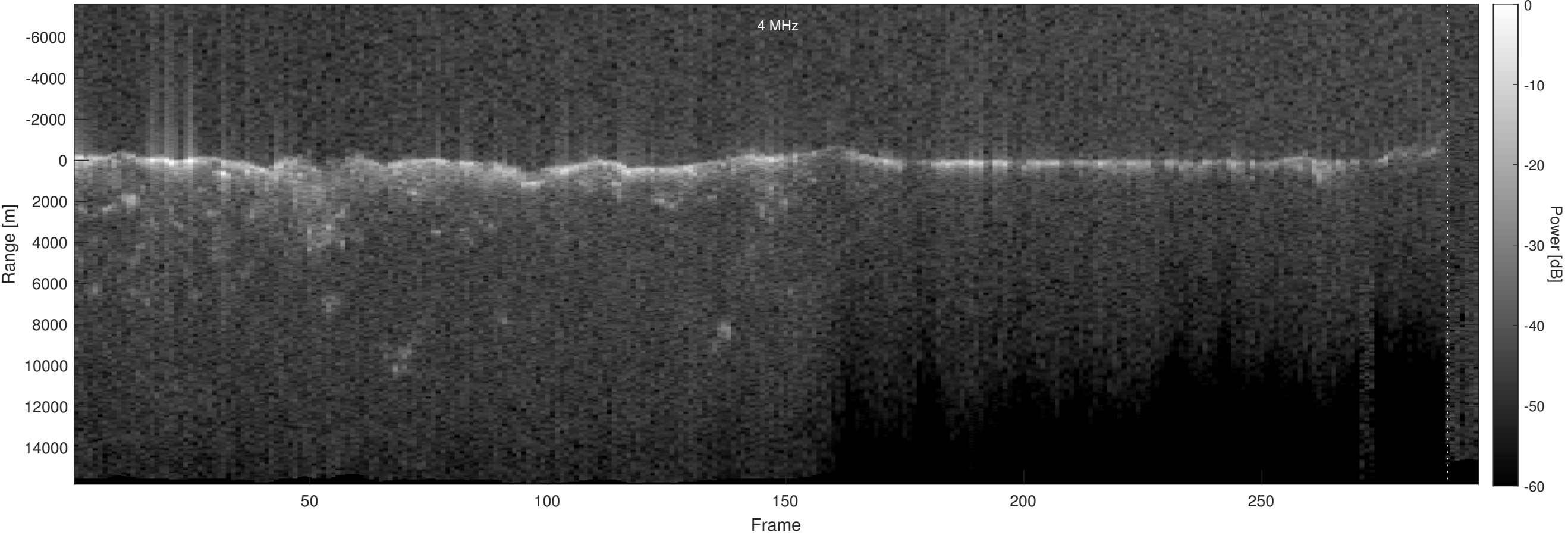
Orbit 14956, Optimized, No Window, Depth-Corrected, Channel 2
