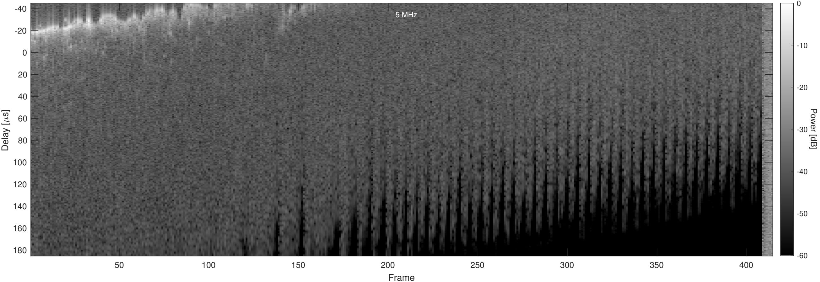
Orbit 14969, Chapman, No Window, Channel 2
